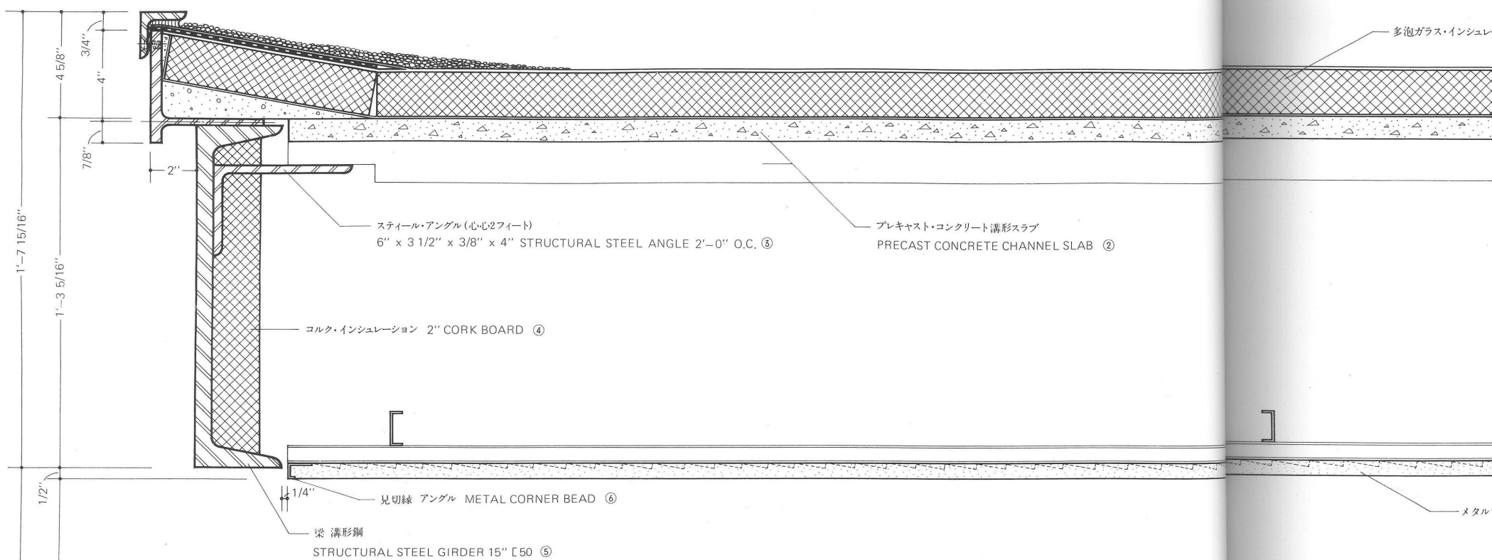
屋根断面図 Section D-D through Roof
