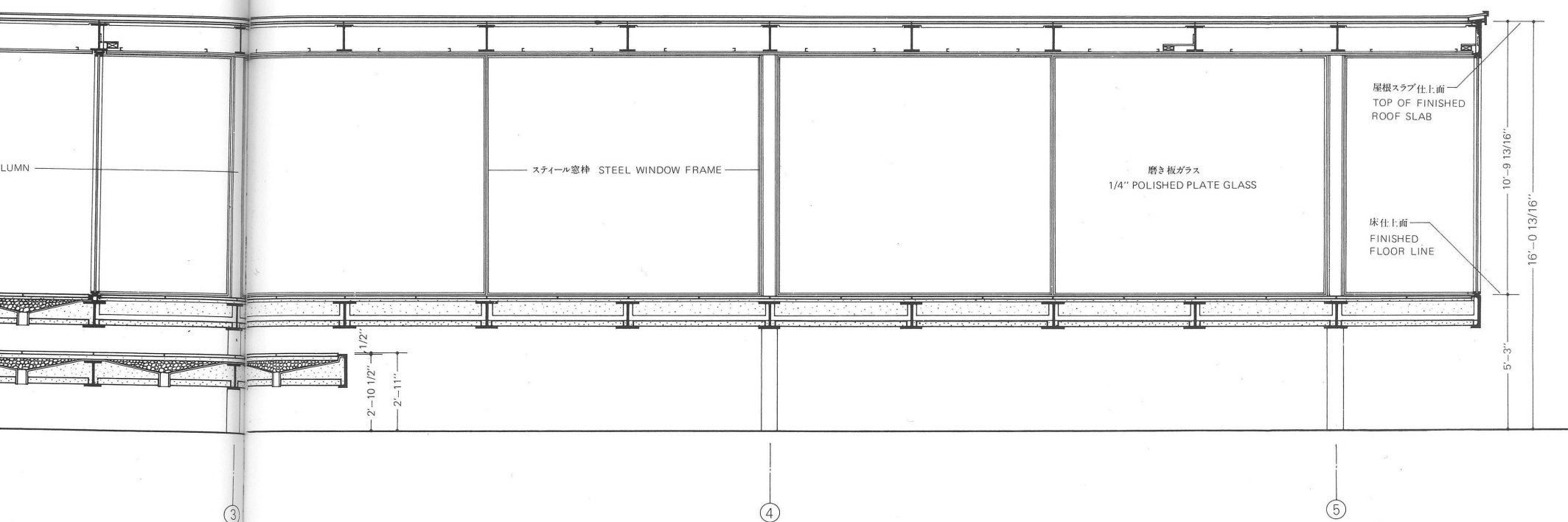
縦断面図 テラスの柱③と④, 住宅の柱④と⑤の間を切って北を見る Longitudinal Section between Column Lines ③ & ④ for Terrace and ④ & ⑤ for House Looking North
