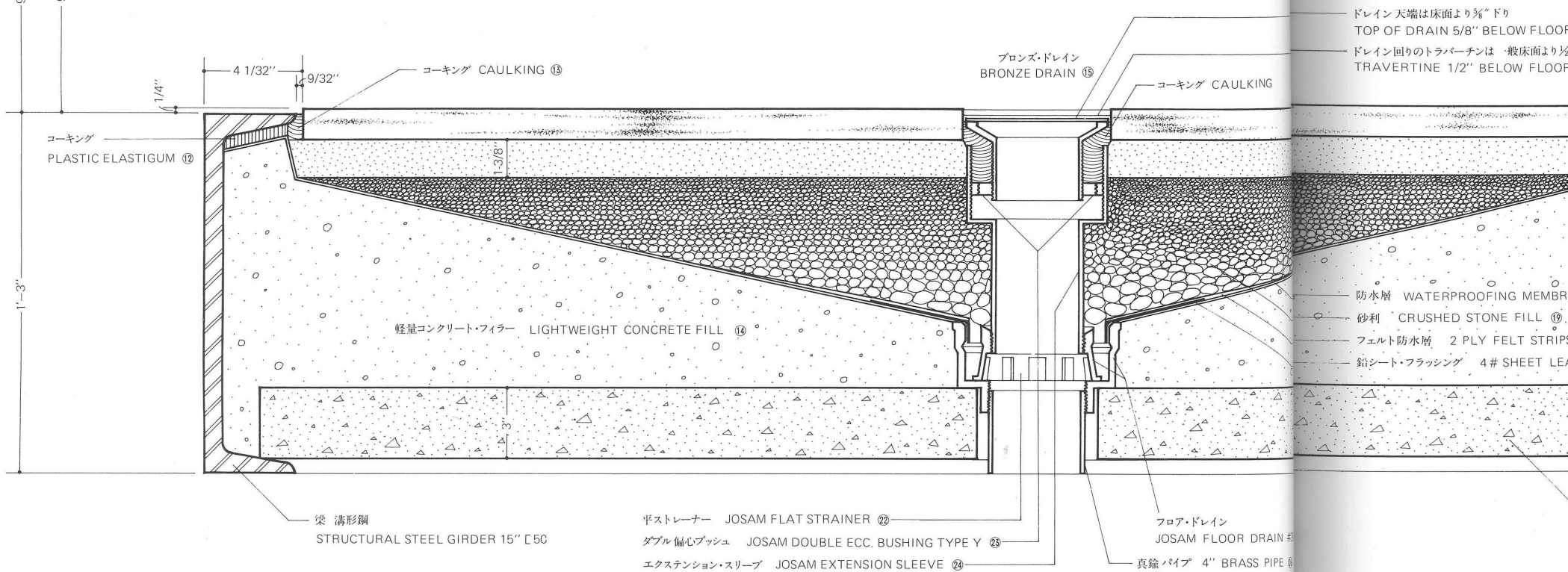
床断面図 Section D-D through Floor
