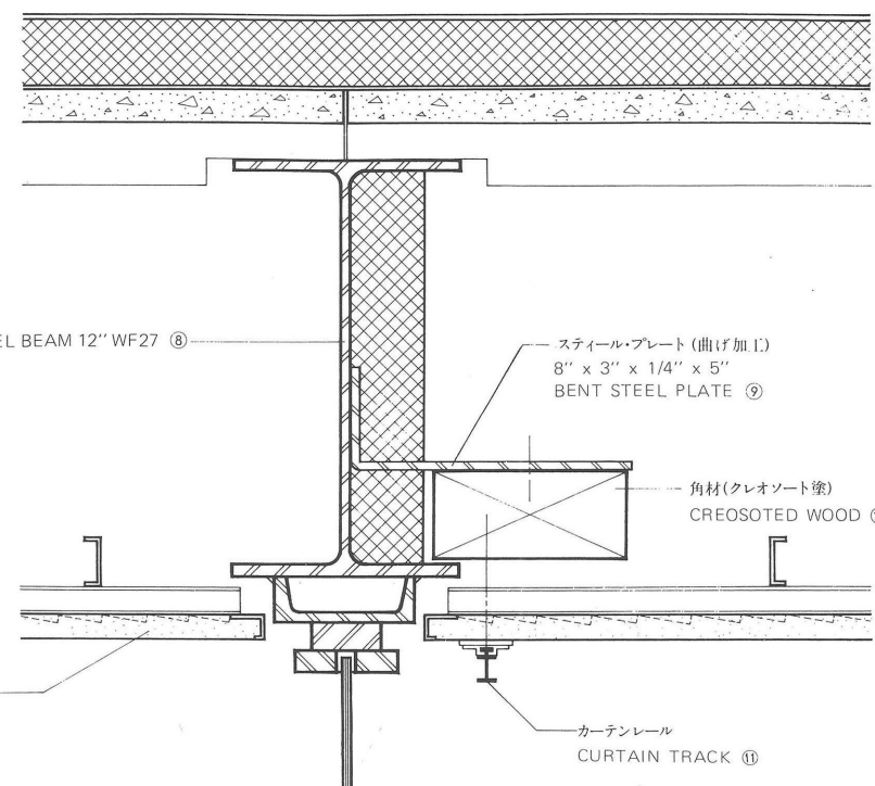
屋根断面図 Section F-F through Roof
