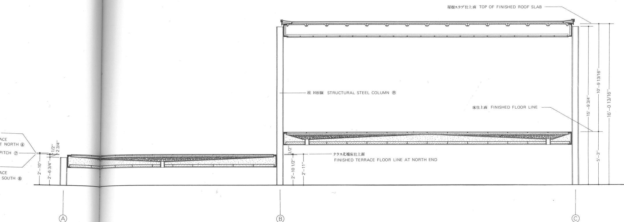
横断面図 柱②と③の間を切って西を見る Cross Section between Column Lines ② & ③ Looking West
