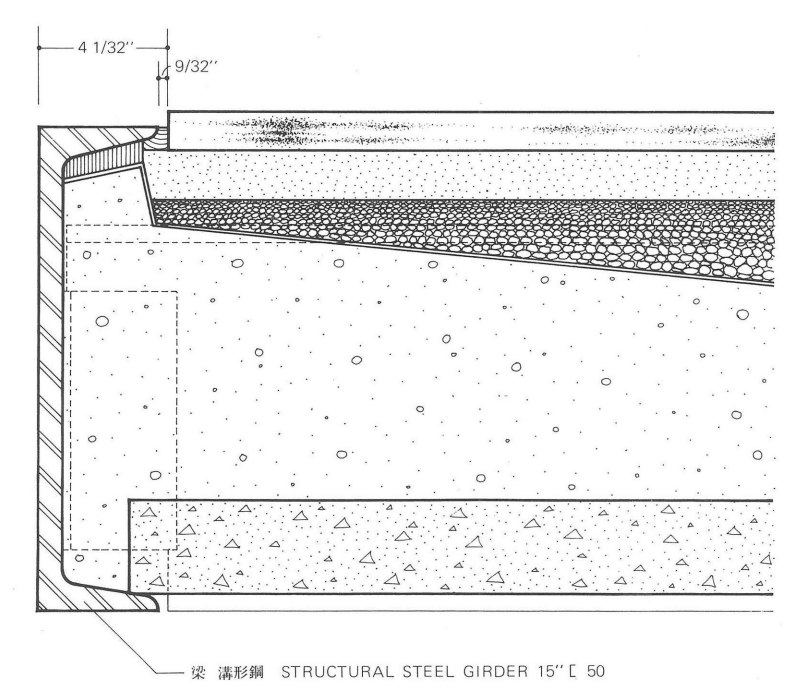
テラス断面図 Section G-G through Terrace
