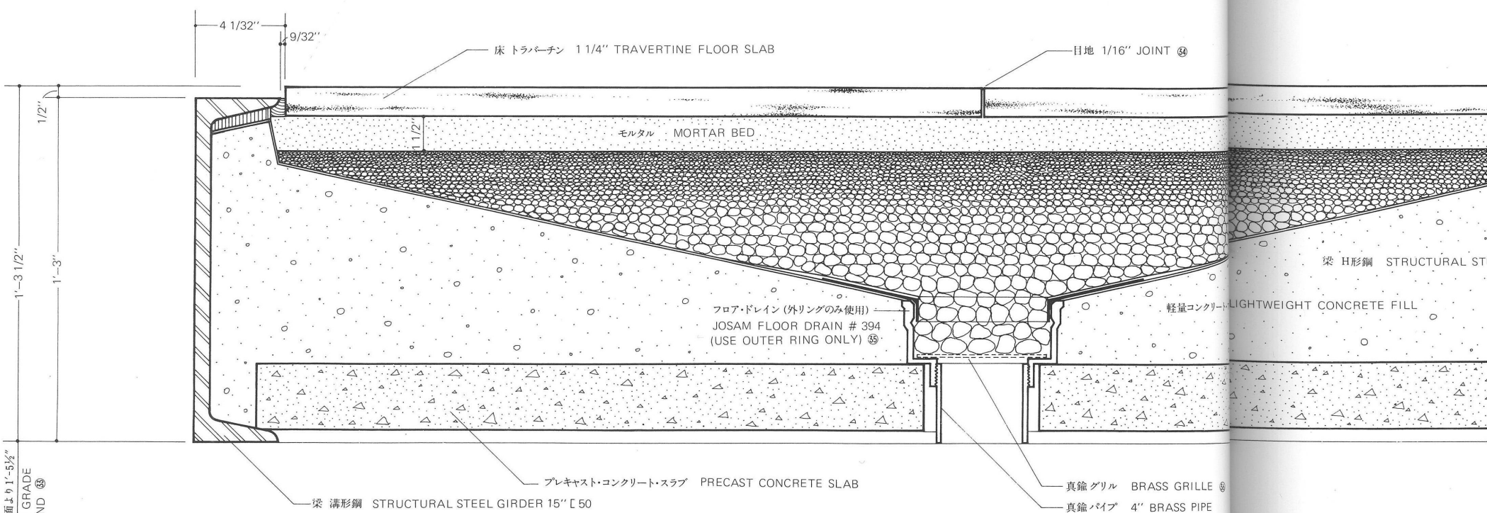
テラス断面図 Section E-E through Terrace
